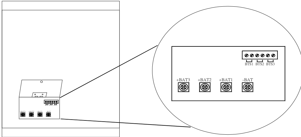
Figure A: Batteries terminals and BTS terminals
